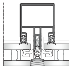
Horizontal Section
