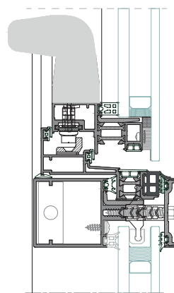
Vertical Section
