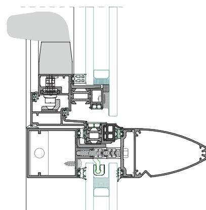
Vertical Section
