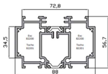
Marco-Hoja-Pilastra 17470
