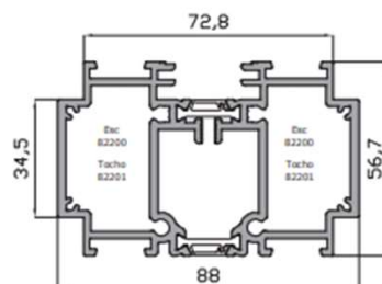
Marco-Hoja-Pilastra Antibimetel 17475
